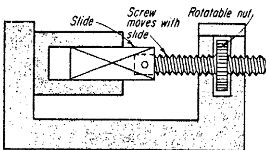
NON-ROTATING SCREW/ROTATING NUT
