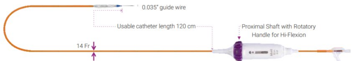
"Navigator" delivery apparatus
